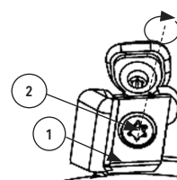
PICTURE E When you reach the axial measure you need, tighten the clamping screw at 4.5Nm (no. 2). Repeat the procedure for each insert.
