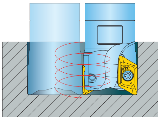
HELICAL MILLING TABLE
