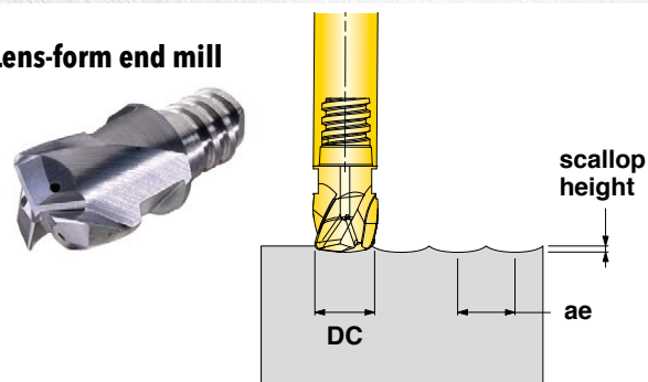
Ball-Nose vs. Lens-Shape Stepover Comparison 0.0002" (0.50mm) Scallop Height
