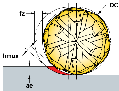
Chip Thinning
