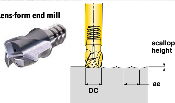
Ball-Nose vs. Lens-Shape Stepover Comparison .0002" (0.50mm) Scallop Height
