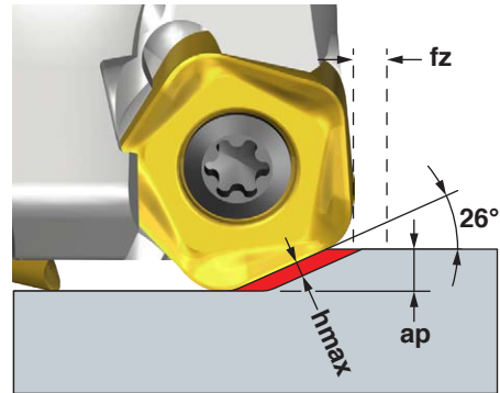
Chip Thinning
