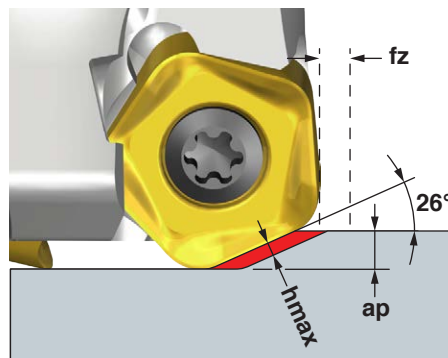
Chip Thinning
