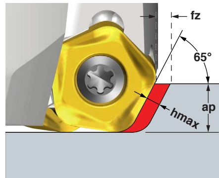
Chip Thinning
