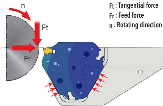
Triangular blade with enhanced rigidity and stable support structure (No vibration)
