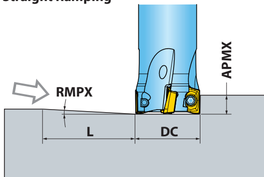
Straight Ramping
