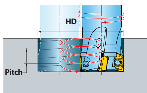
Helical Ramping
