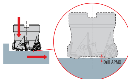
Drill Mill
