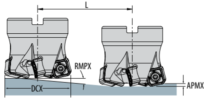
Straight Ramping
