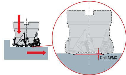
Drill Mill
