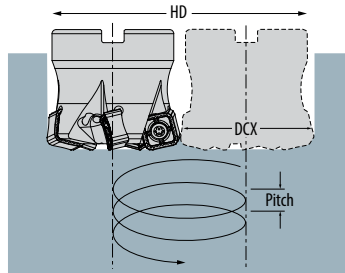
Helical Ramping
