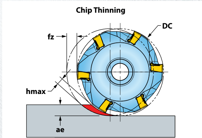
* Chip Thinning Calculator is recommended to ensure hmax falls within fz range.
